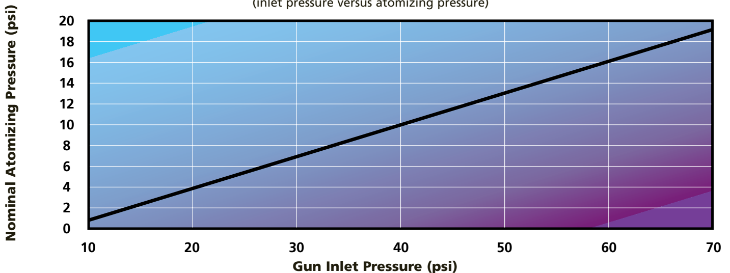
Atomizing Air Pressure (inlet pressure versus atomizing pressure)
